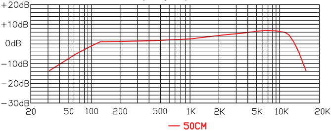
Frequency Respond
